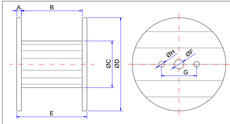
M800, M1000, M1250 wooden spool
